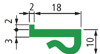
■ GP 251 ZK Profile 40M/Roll 型墊片 40M/捲
