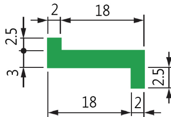
■ GP 241 Z Profile 80M/Roll 型墊片 80M/捲
