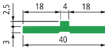
■ GP 242 T Profile 80M/Roll 型墊片 80M/捲
