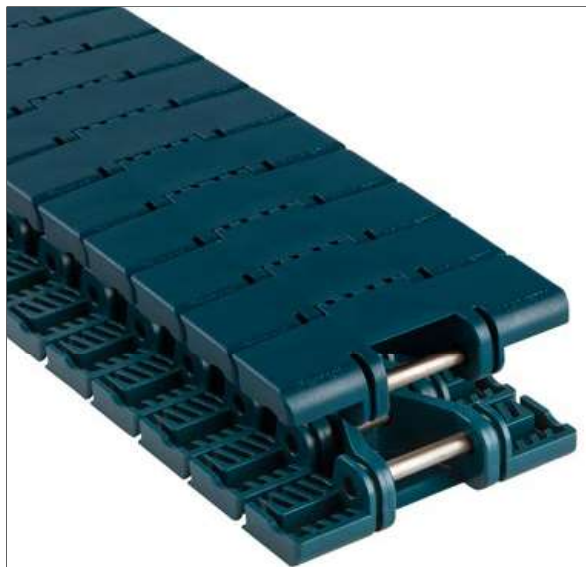
Photo shows 1040 FTM TableTop Chain with Magnetflex Retention molded in XLG material.
