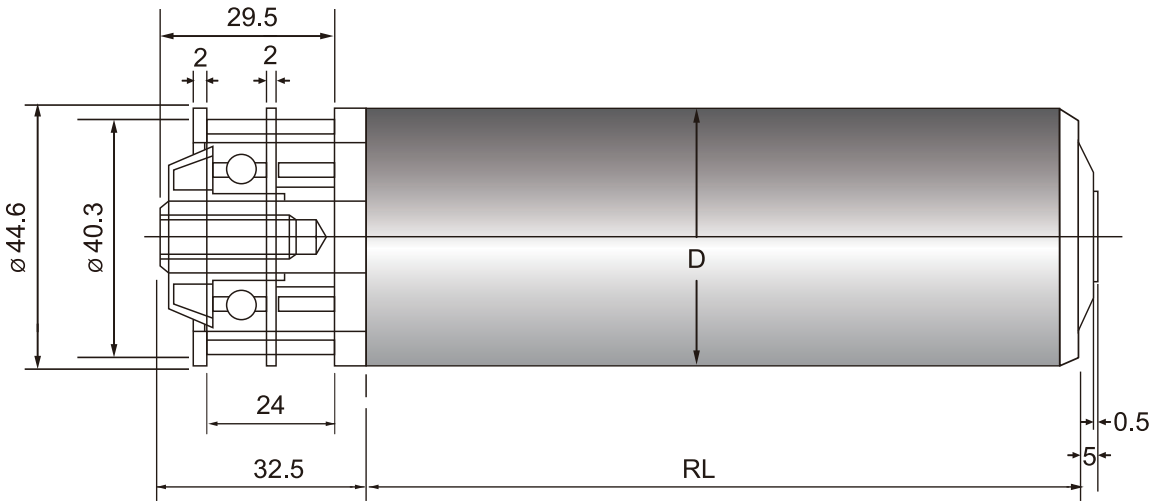
T5*26T-2時規皮帶滾輪
