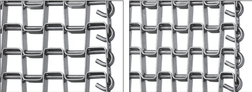
H4 - 1" x 1" Mesh, Clinched Selvage H5 - 1/2" x 1" Mesh, Clinched Selvage
