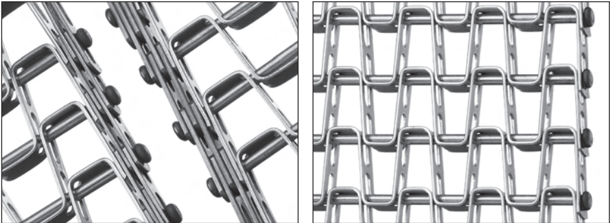
T1 - 1" x 1" Mesh, Welded Selvage Shown with 0.062" and 0.090" thick double reinforcing links
