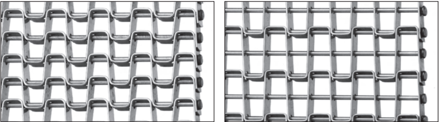
S5 - True 1/2" x 1/2" Mesh, Welded Selvage S6 - 1/2" x 1" Modified Mesh, Welded Selvage
