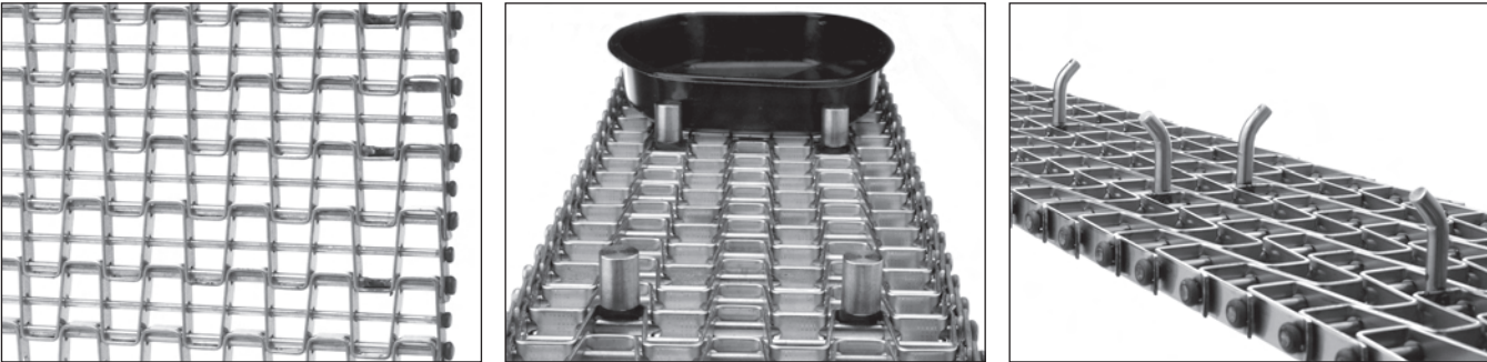
Narrow Mesh Nut Harvester Belting Custom Filling Station Belt Belt with Custom Fixture
