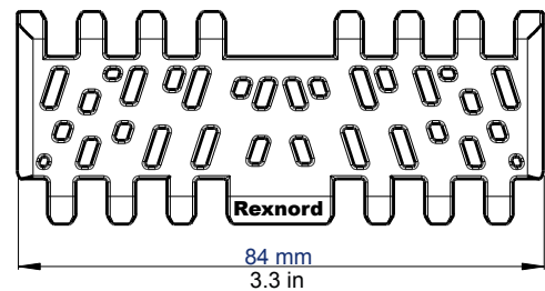
Rexnord 1001 Series Flush Grid MatTop Chain top view
