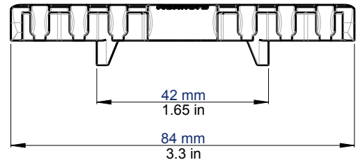
Rexnord 1001-84mm Series MatTop Chain front view
